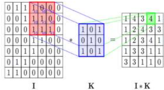
Fig 2. Convolutional layer
