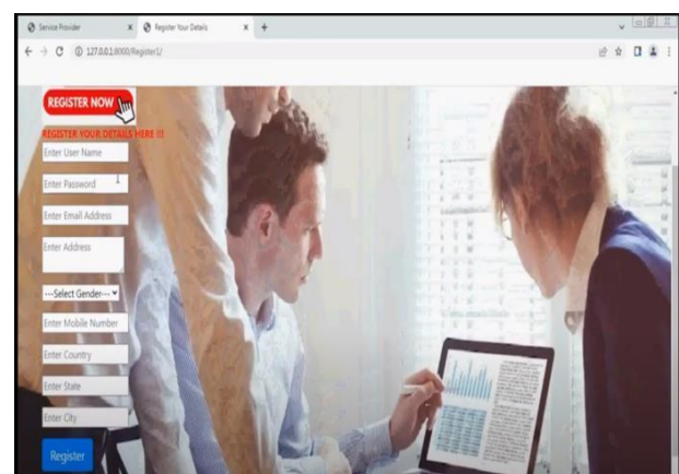
Fig.4. Register details.
