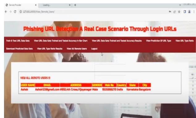
Fig.3. User details.
