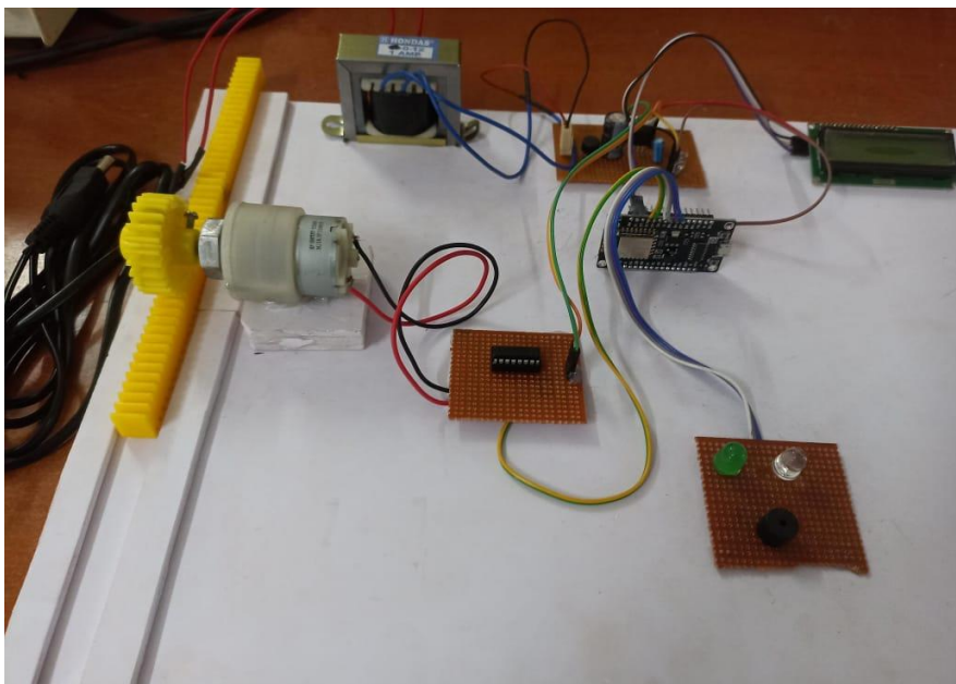
Figure.3 Real time connections overview
