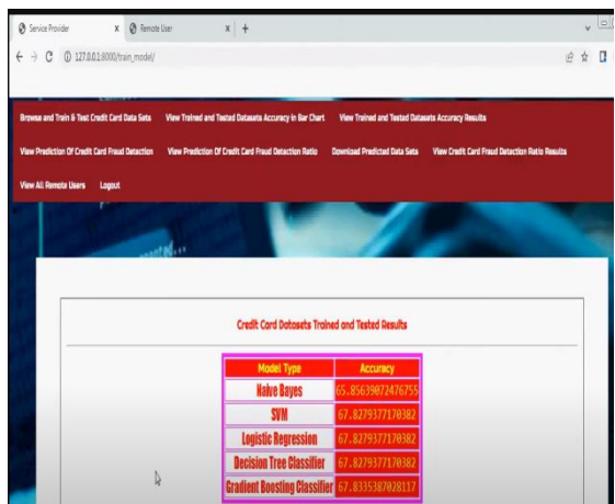
Fig.7. Algorithms applied.
