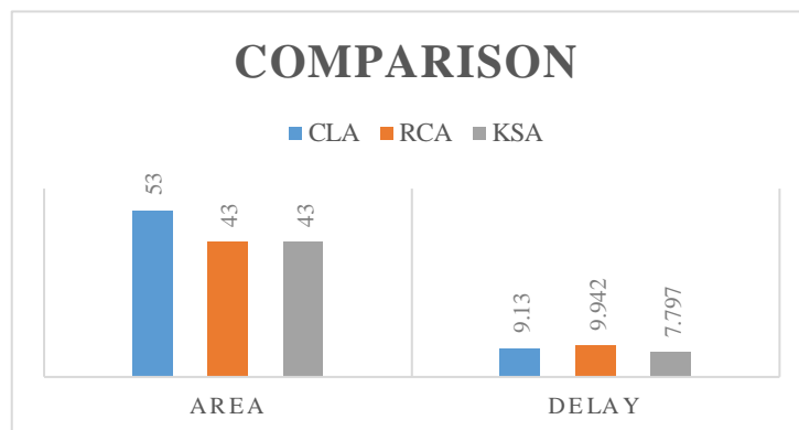
Fig 4: Comparison of various adders in terms of area and delay
